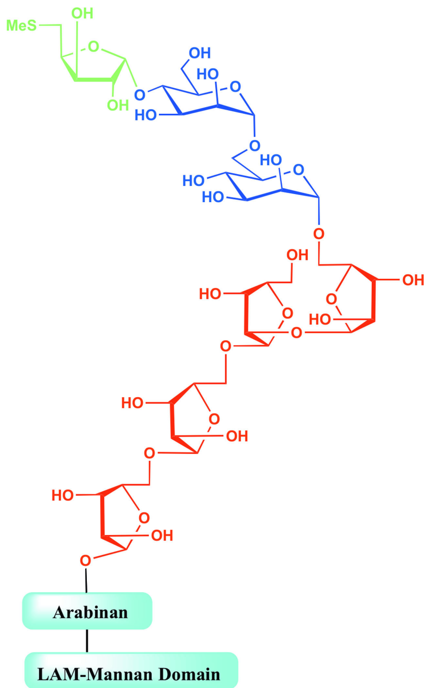
Figure 1. Representation of the non-reducing arabinan termini of M. tuberculosis ManLAM
