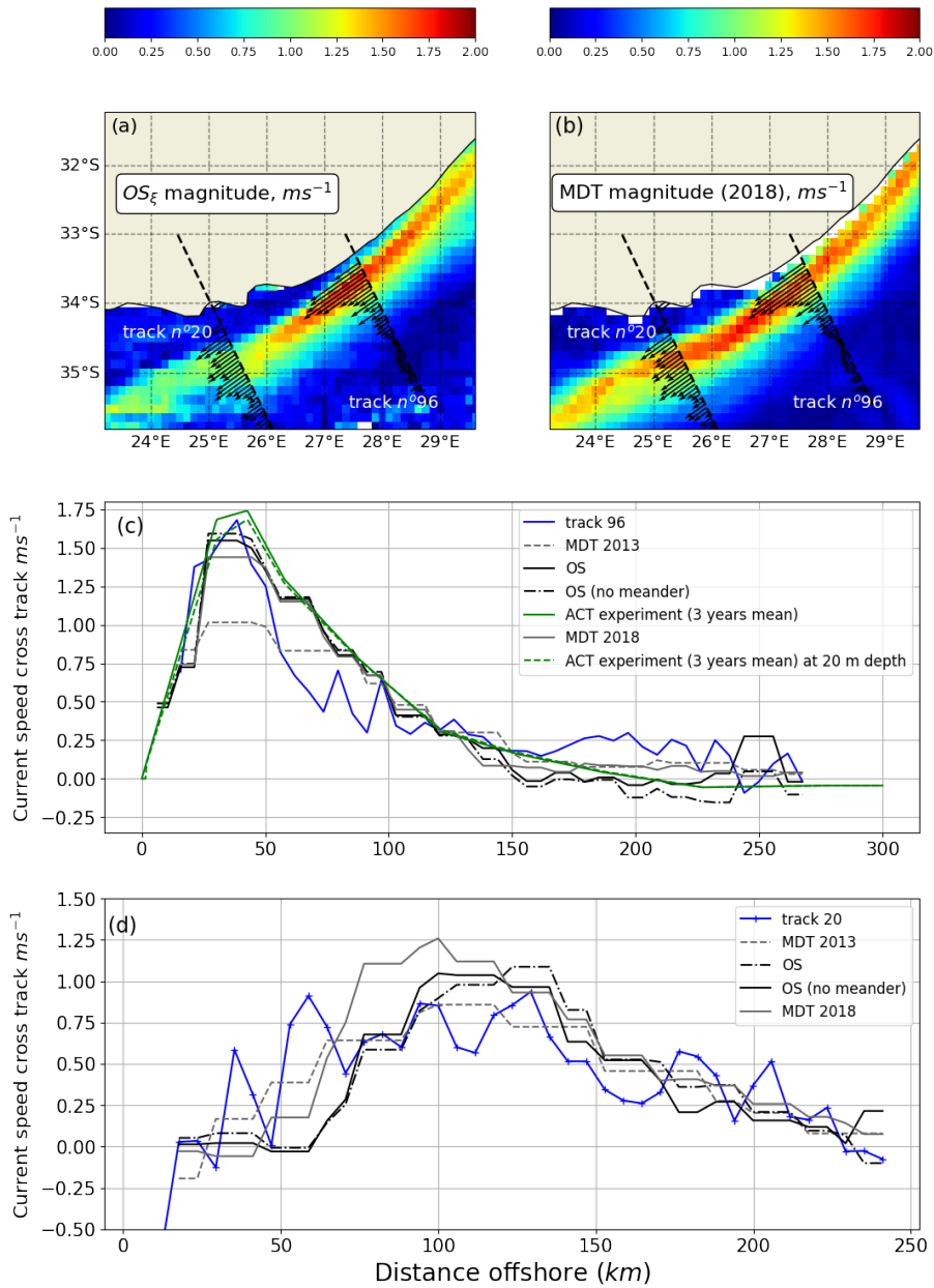
Figure 9: (a) Time average of the magnitude of our ocean surface current estimates. (b) Time average of the magnitude of the oceanic current derived from the MDT 2018. Quivers represent the time average for the Along-Track geostrophic velocities for the Jason-2 tracks 20 and 96. (c) In blue, the cross-track velocity from Jason-2 track 96 for the year 2016 (mean of 20 altimeter geostrophic velocities). In green, the cross-track surface velocities from the gridded dataset of the ACT experiment averaged over 3 years for the surface (full line) and at 20 meters depth (dashed line). The oceanic surface current velocity is represented by a black full line for the year 2016 and current velocities associated to the two MDT estimates are shown in gray (full line for 2018, dashed line for 2013). (d) Same as (c) but for the altimeter Jason 2 track 20.
