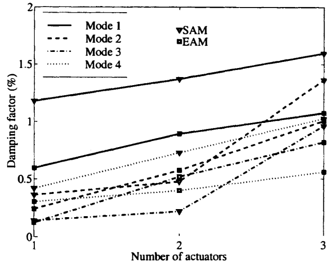
Figure 8. Variation of the first four natural bending modes damping with number of actuators.
