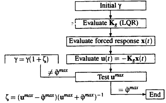
Figure 4. Algorithm for control gain evaluation ( 2\tilde{\phi}_f^{max} = \tilde{\phi}_c^{max} = 200 V).
