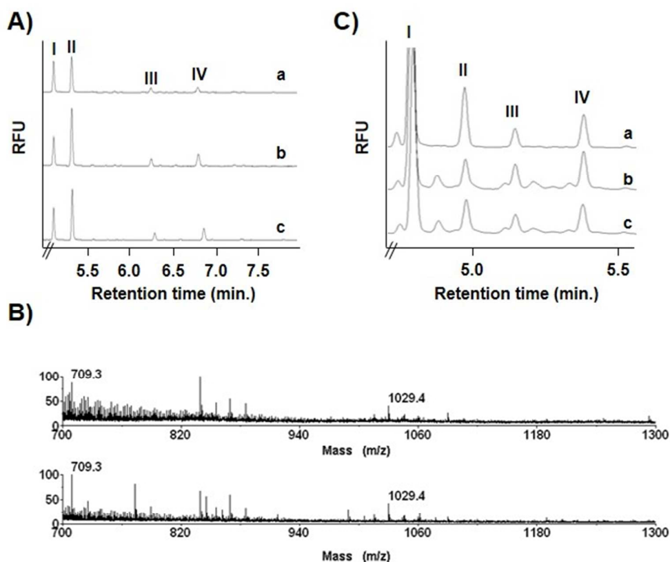
Figure 5. Structural analysis of compound X arabinan (A, B) and mannan (C) domains. A, B) Digestion of arabinan domain (10 \mu\text{g} of compound X) by endoarabinanase from Cellulomonas gelida monitored by CE-LIF (A) and MALDI-TOF MS analysis (B). A) I, Internal Standard-APTS; II, Ara2-APTS; III, Ara4-APTS; IV, Ara6-APTS; a, compound X; b, LAM from M. smegmatis ; c, co-injection. B) MALDI-TOF MS analysis in positive ion mode of the permethylated products of hydrolysis of LAM (upper spectrum) and Compound X (lower spectrum) (50 \mu\text{g} of each). Ions at m/z 709.3 correspond to Ara4 motif and m/z 1029.4 correspond to Ara6 motifs. C) Mannan core degree of branching determined by acetolysis treatment (10 \mu\text{g} of compound X). I, Ara-APTS; II, Man-APTS; III, Internal Standard-APTS; IV, Man- \alpha(1\rightarrow2) Man-APTS; a, compound X; b, LAM from M. smegmatis ; c, co-injection.
