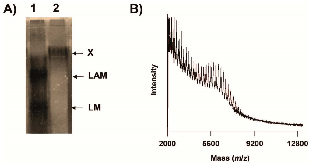
Figure 4: DOC-PAGE (A) and MALDI-TOF MS (B) analyses of compound X. A) 10 \mu\text{g} of the M. smegmatis glycans and lipoglycans fraction were loaded on the gel before (lane 1) or after alkali-treatment (lane 2). The gel was revealed by zinc sulphate negative staining. B) Linear MALDI-TOF MS spectrum in the positive mode of permethylated compound X.
