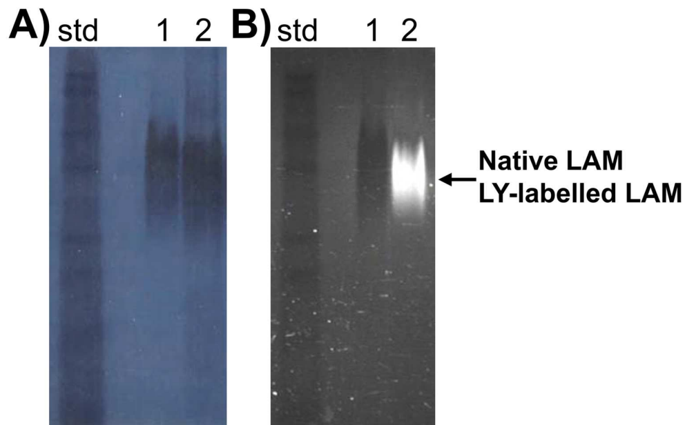
Figure 2: DOC-PAGE migration of native and LY-labelled LAM. 5 \mu\text{g} of native (lane 1) and LY-labelled (lane 2) LAM were submitted to DOC-PAGE migration. The same gel was revealed first by zinc sulphate negative staining (A) and then by UV (B). std, protein ladder.
