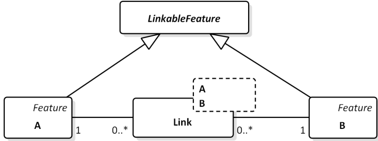
Figure 3: GenLinkable : Conceptual model for linking features.
