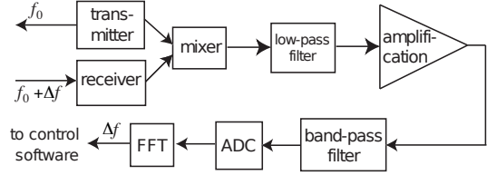
Fig. 7. Frequency acquisition process
