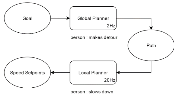
Figure 1: Control Architecture. The global planner receives a goal and produces a path at a 2Hz frequency. This path is sent to the local planner which computes the speed setpoints to be sent to the controller at a 20Hz frequency.
