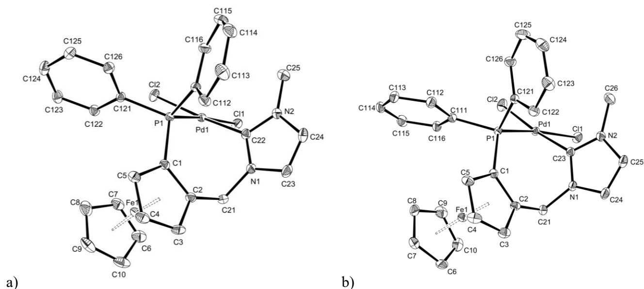
Figure 1. ORTEP representations of complexes 2a-rac (left) and 2a-(R) (right). Ellipsoids are shown at the 30% level. All hydrogens are omitted for clarity. Selected bonds (Å) and angles (°), 2a-rac : C(22)-Pd(1) = 1.991(3), P(1)-Pd(1) = 2.2444(8), Cl(1)-Pd(1) = 2.3614(9), Cl(2)-Pd(1) = 2.3397(8), C(22)-Pd(1)-P(1) = 84.95(9), C(22)-Pd(1)-Cl(1) = 88.24(9), P(1)-Pd(1)-Cl(2) = 95.06(3); 2a-(R) : C(23)-Pd(1) = 1.976(3), P(1)-Pd(1) = 2.2472(10), Cl(1)-Pd(1) = 2.3665(9), Cl(2)-Pd(1) = 2.3481(9), C(23)-Pd(1)-P(1) = 86.61(10), C(23)-Pd(1)-Cl(1) = 83.61(10), P(1)-Pd(1)-Cl(2) = 98.97(3).
