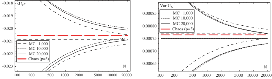
Fig. 12. Convergence of the mean and variance of the displacement U_x at point A ( \delta_I = 0.2 and \delta_{II} = 0.25 ): comparison between the LATIN solution and the Monte Carlo solution for a confidence level of 0.95 ( n = 2 ) for various sample sizes.
