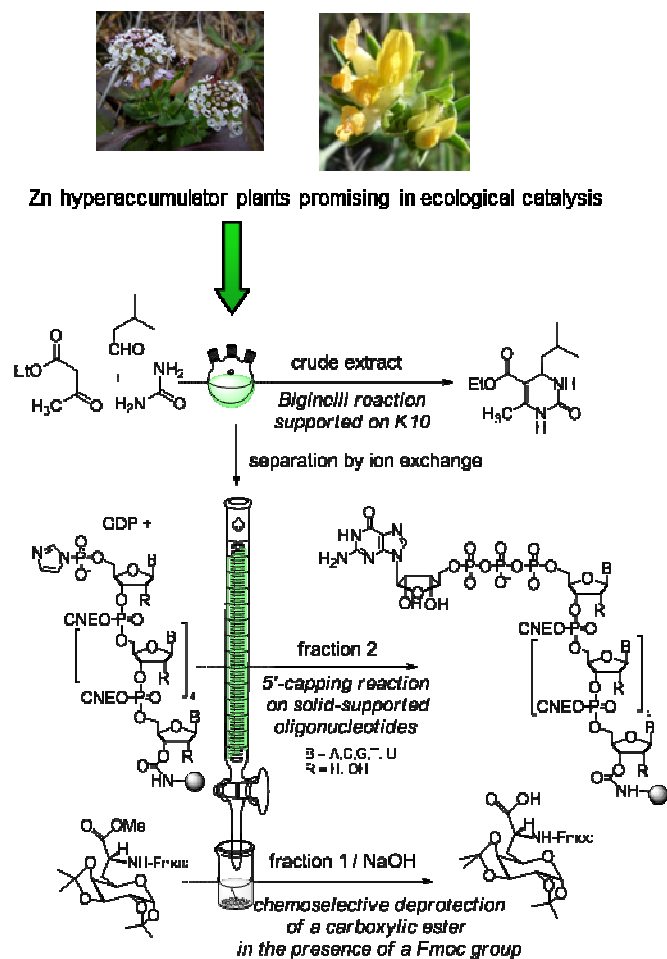
Fig. 7. Synthetic applications of ecological catalysts in the transformations of biomolecules
