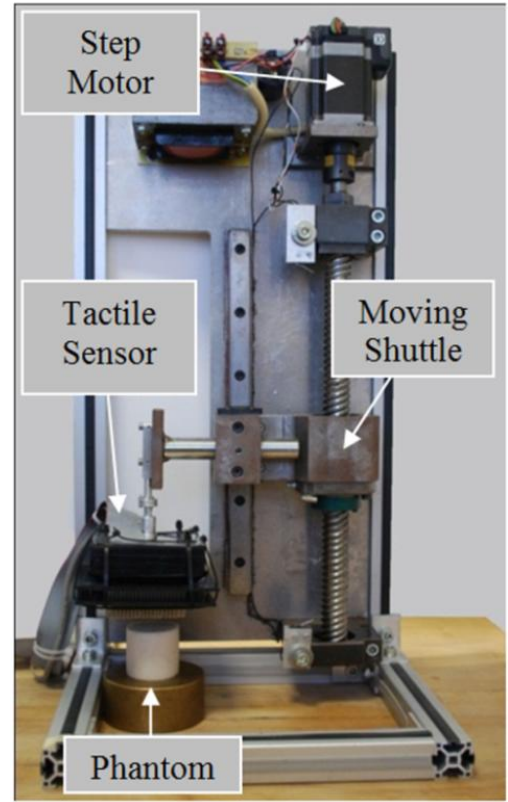
Fig. 7. The mechanical compression device used in our study to characterize material properties of the silicon samples and to evaluate the performance of our tactile sensor.
