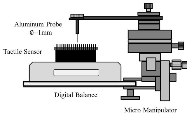
Fig. 4. a) The calibration set-up for the tactile sensor. b) The calibration curve of a sensor element used in the tactile imaging system.
