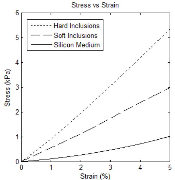
Fig. 8. The stress versus strain curve for the hard inclusion ( E = 91 kPa at 1% strain and E = 107 kPa at 5% strain), for the soft inclusion ( E = 56 kPa at 1% strain and E = 60 kPa at 5% strain), and for the tissue-like silicon medium ( E = 11 kPa at 1% strain and E = 20 kPa at 5% strain).
