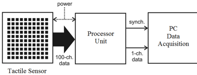
Fig. 3. Data acquisition units of the proposed tactile imaging system.
