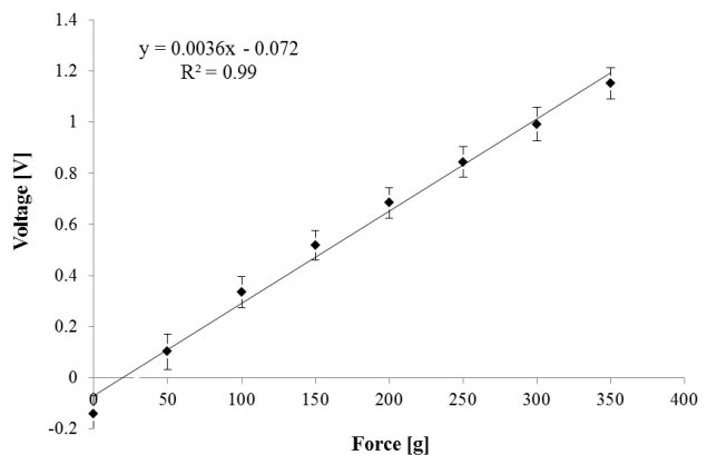
Fig. 4. a) The calibration set-up for the tactile sensor. b) The calibration curve of a sensor element used in the tactile imaging system.
