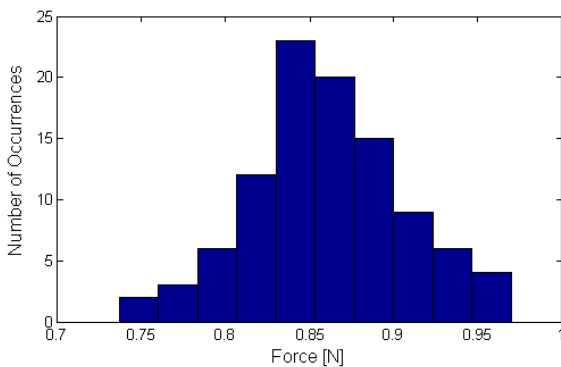
Fig. 2. A histogram of the force values measured at the center pixel for the compression depth of 19 mm. The mean force, the standard deviation and the coefficient of variation are 0.86 N, 0.05 N, and 5.8%, respectively.
