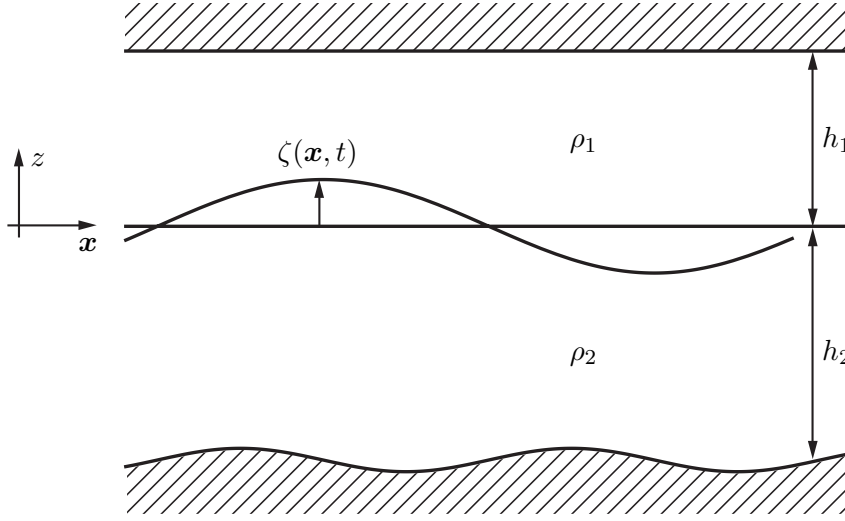
Figure 1.1: Interfacial gravity waves
