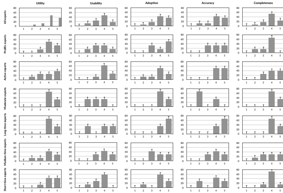
Fig. 17. Satisfaction and effectiveness metrics results.
