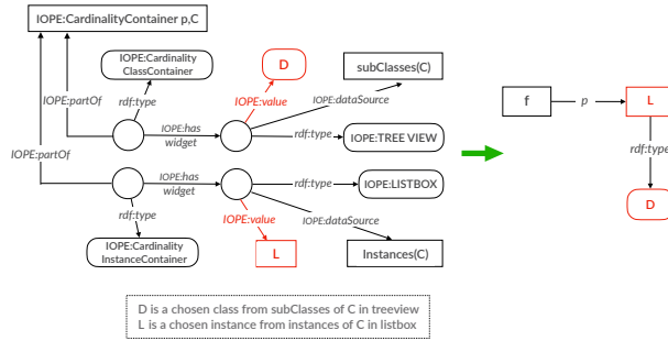
Fig. 14. Binding rule for a selected class D in a IOPE:TREEVIEW and selected instance(s) L from a IOPE:LISTBOX widget
