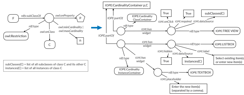
Fig. 9. Mapping rule for a Cardinality constraint where subClasses(C) and instance(C) are not empty
