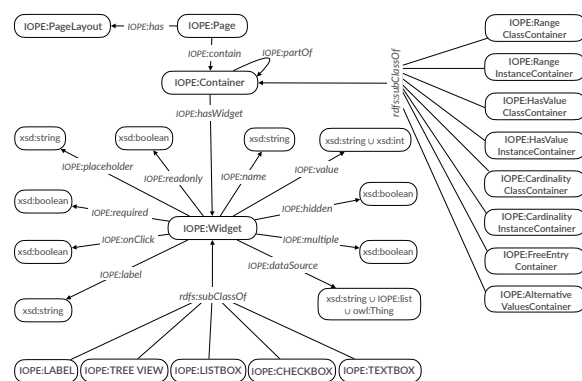
Fig. 5. The IOPE Web form ontology
