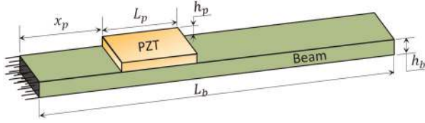
Figure 3. Cantilever beam with one piezoelectric patch. PZT: lead zirconate titanate.
