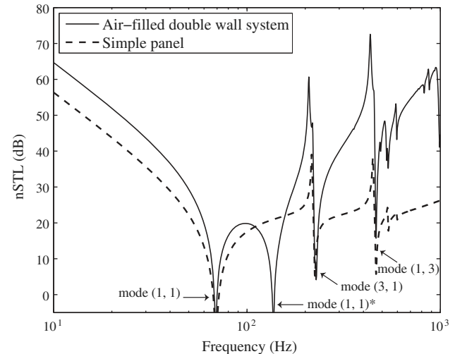
Fig. 5. Comparison of the normal incidence sound transmission (nSTL) through an air-filled double panel and a simple panel.
