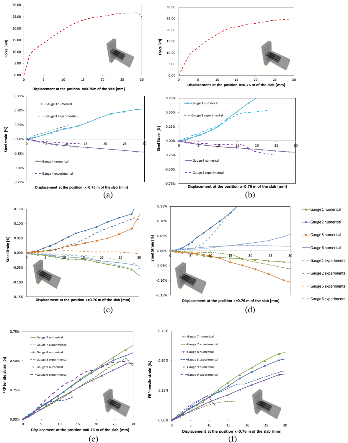
Figure 10 - Comparison of experimental and numerical strain (Steel and FRP) for the RC1-CFRP-ALc38-At and RC1-CFRP-Ali38-At wall/slab connections
