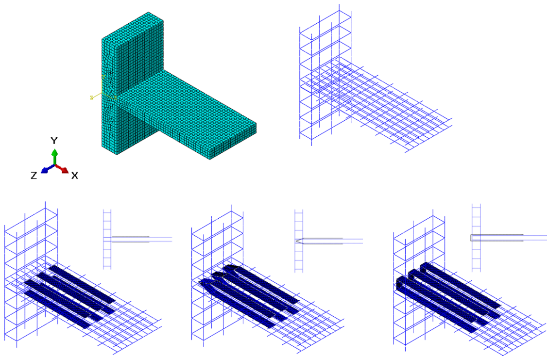
Figure 4 - The FEM model used for the RC wall/slab connections and details of steel rebars and FRP in each connection
