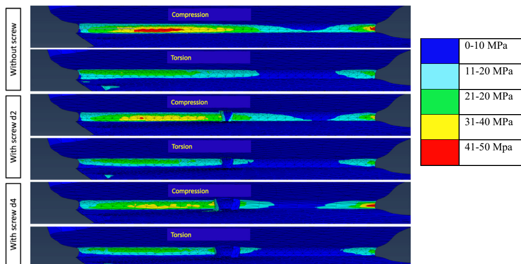
Fig. 5. Visualization of the equivalent Von Mises stress zones in the lateral hinge (sagittal section).
