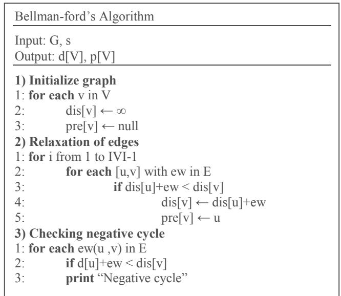
Fig. 4. Bellman-ford's Algorithm
