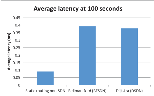
Fig. 9. The average latency
