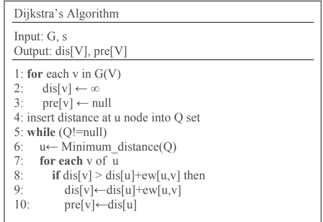
Fig. 3. The Dijkstra's Algorithm
