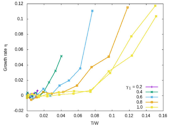
Figure 5. Growth rate versus Ostriker–Peebles parameter for six sets of models with q = -6 , 0 \le \alpha \le 1 and various \gamma_1 . Note that two realizations have been computed for the case \gamma_1 = 1 , which gives an impression of the accuracy with which the growth rate has been estimated.
