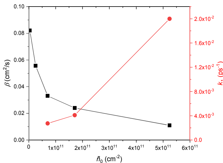
38 39 40 41 42 43 44 45 46 47 48 49 50 51 52 53 54 55 56 57 58 59 60 Figure 3. Evolution of the effective bimolecular AR rate \beta (black squares) and of the effective linear AR rate constant k_1 (red dots) with the initial exciton density extracted from the TR-PL
