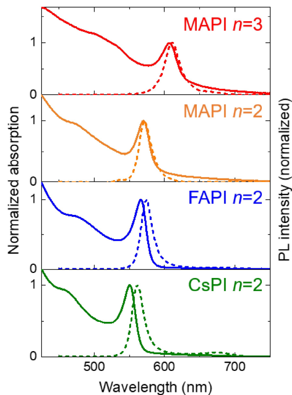
13 14 15 16 17 18 19 20 21 22 23 24 25 26 27 28 29 30 31 32 33 34 35 36 37 38 39 40 41 42 43 44 45 46 47 48 49 50 51 52 53 54 55 56 57 58 59 60 Figure 1. Absorption (full line) and photoluminescence (dashed line) spectra of colloidal perovskite NPLs of two monolayers (CsPI, FAPI, MAPI n=2 ) and three monolayers (MAPI n=3 ).
