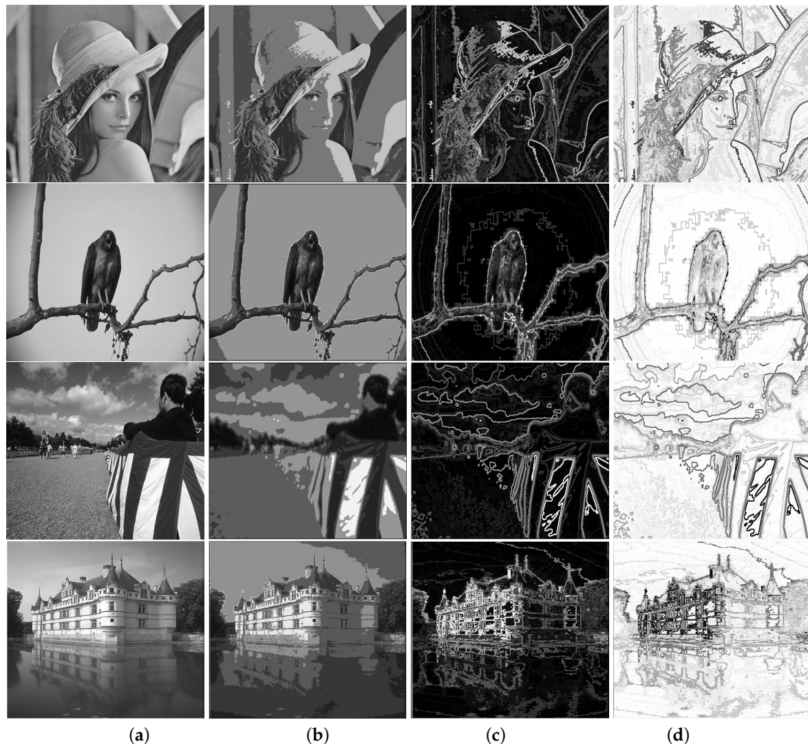
Figure 3. Z-coded images. (a) original images. Segmented images obtained by combining intersection with (b) max(max) (c) min(max) (d) max(min).
