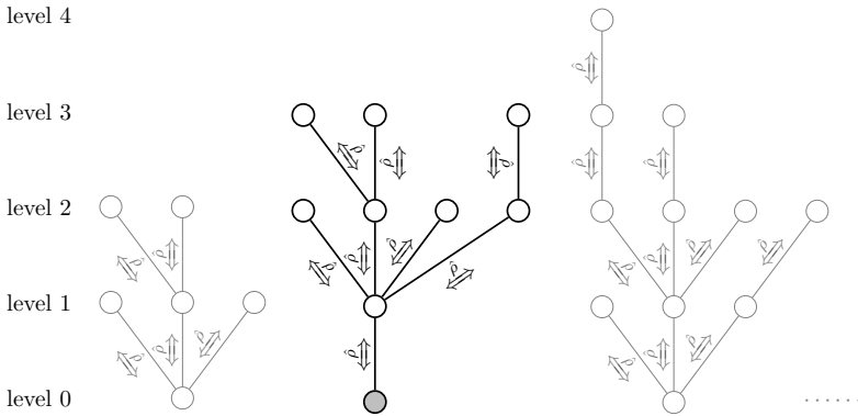
Figure 6.1. The forest structure of (\Gamma \setminus \widehat{\Gamma}^+, \mathcal{E}_{\hat{\rho}}) . In each tree, a root node is fixed, and the other nodes are organised by levels corresponding to their distance to the root. One of the trees is emphasized, as well as the chosen root.
