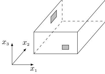
FIGURE 3. The geometry of the boundary control problem in 3D. The control domain is the part of the boundary which is represented in gray.
