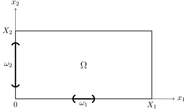
FIGURE 1. Domain \Omega and control region \gamma = (\omega_1 \times \{0\}) \cup (\{0\} \times \omega_2)
