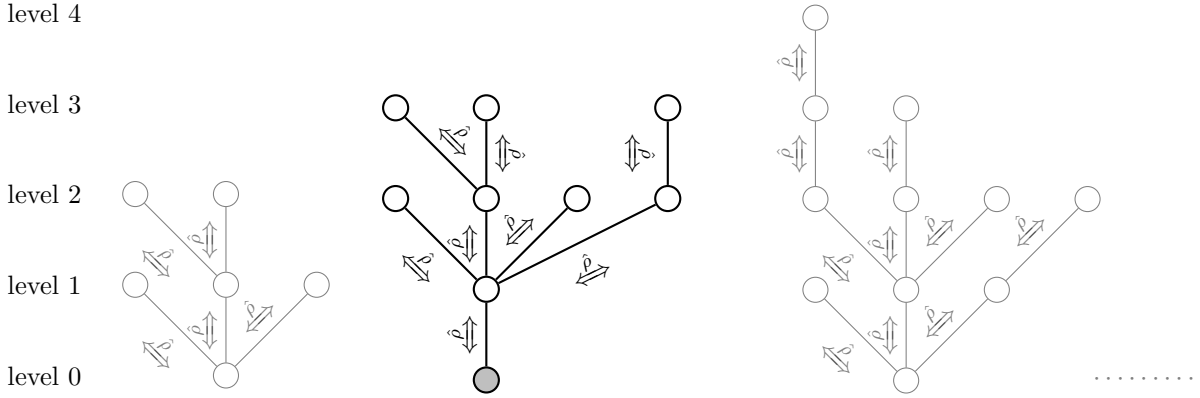
FIGURE 2. The forest structure of (\Gamma \setminus \hat{\Gamma}^+, \mathcal{E}_{\hat{\rho}}) . In each tree, a root node is fixed, and the other nodes are organised by levels corresponding to their distance to the root. One of the trees is emphasized, as well as the chosen root.
