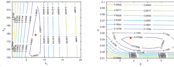
Fig. 1 Contour plot of the spectral radius of the iteration matrix T(\widetilde{\Sigma}_1, \widetilde{\Sigma}_2) with \widetilde{\Sigma}_i = s_i I (left) and of T(\widetilde{\Sigma}_1, \widetilde{\Sigma}_2) with \widetilde{\Sigma}_i = pI + qH (right). The red crosses are the parameters obtained through Algorithm 1.
