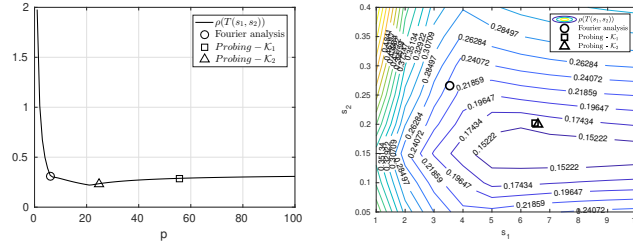
Fig. 3 Comparison between the optimized parameters obtained through Fourier analysis and Algorithm 1 for single sided Robin boundary conditions (left) and double sided Robin boundary conditions (right).
