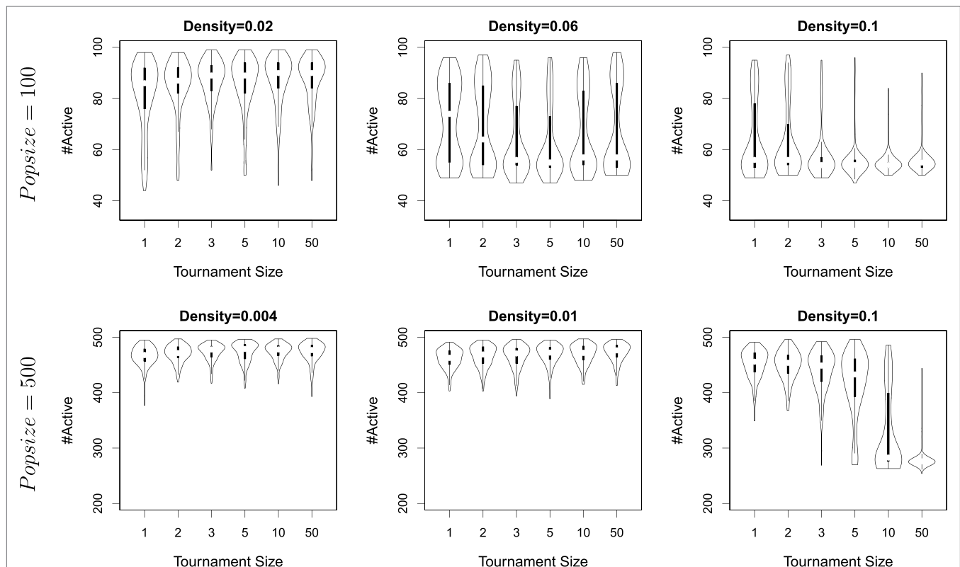
FIGURE 5 | The number of agents alive at the end of a simulation for different densities, different tournament sizes (from 1 to 50), and population sizes (100 and 500). Each violin plots is built from the result of 160 independent runs.
