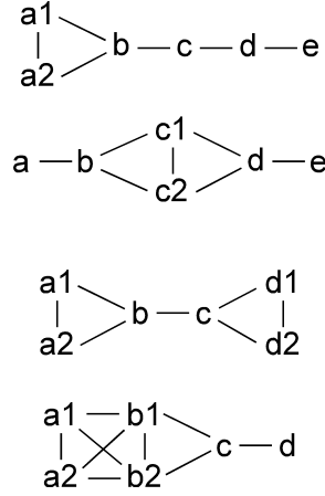
Fig. 4: The bounds of Proposition 5.5(3).
