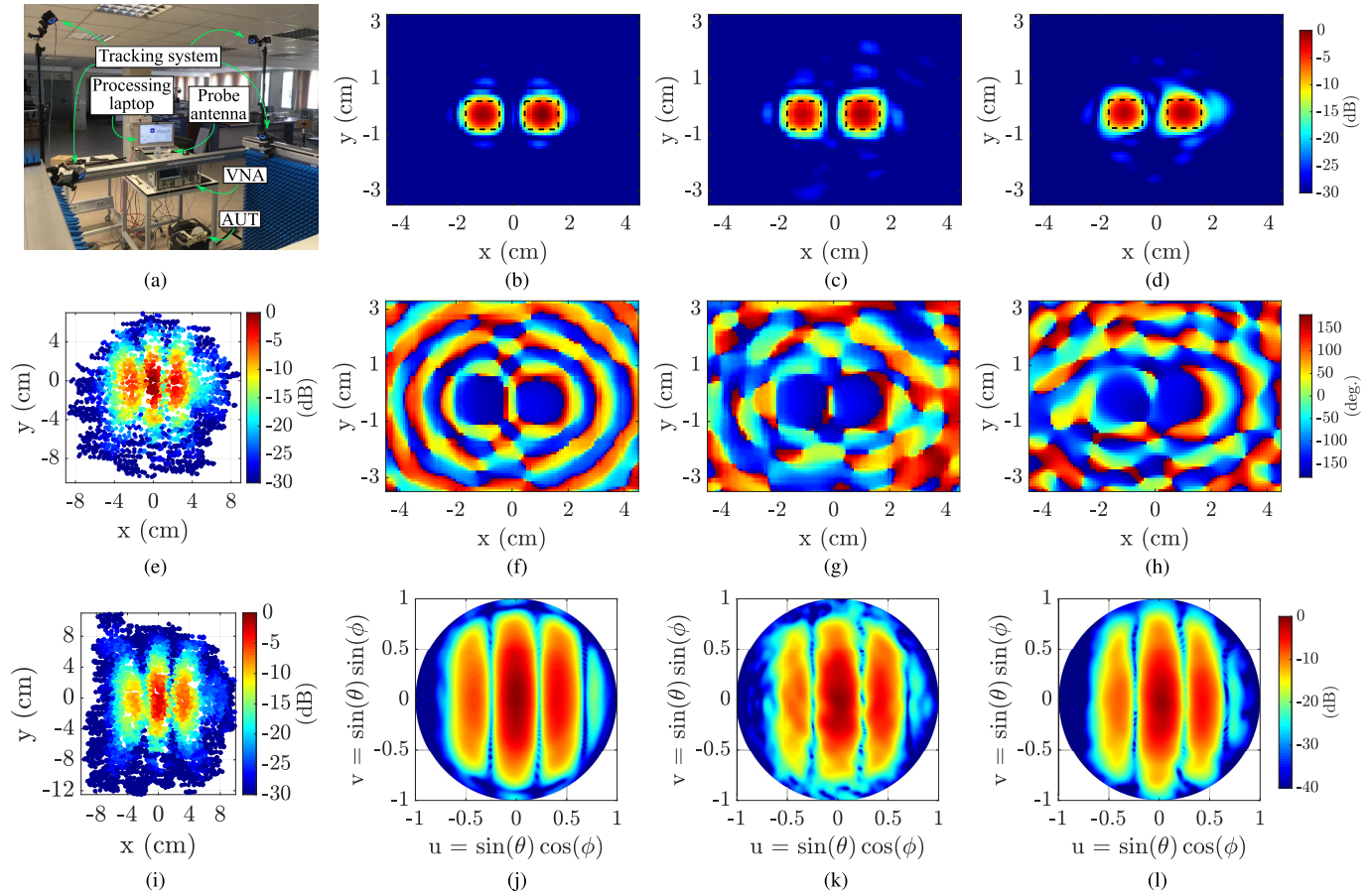
Fig. 3. (a) Setup for the Ka -band measurements. (b) Normalized amplitude and (f) phase of the computed equivalent currents distribution and (j) UV-representation of the retrieved radiation pattern obtained using the standard planar range. The same using (c), (g), and (k) amplitude and phase measurements acquired performing a freehand scan and (d), (h), and (l) using amplitude-only information and the proposed system. Normalized amplitude of the NF samples corresponding to (e) acquisition volume closest to the AUT aperture and (i) farthest one.
