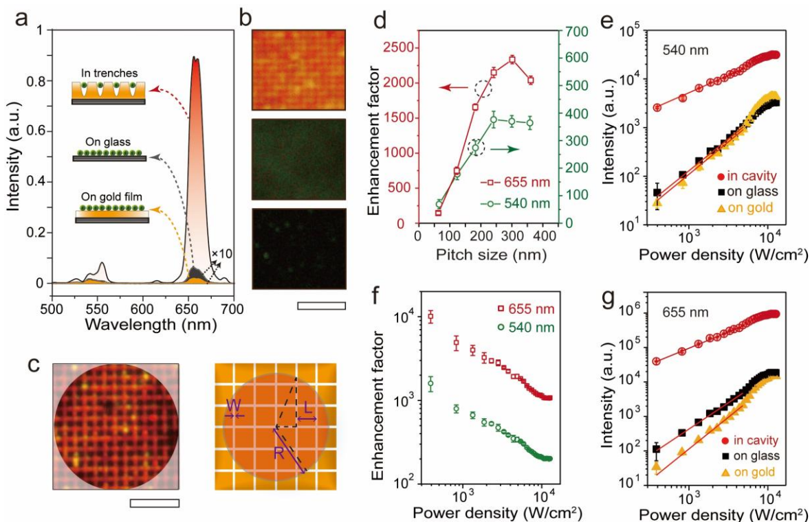
Figure 3. Luminescence enhancement of UCNPs coupled to plasmonic nanotrenches. (a, b) Upconversion luminescence spectra and corresponding fluorescence images of UCNPs assembled within gold nanotrenches with 300-nm pitch (top), on a glass substrate (middle), and on an unpatterned gold film (bottom). Scale bar: 3 \mu\text{m} . (c) Photoluminescence image (left) of UCNPs embedded in a gap-mode nanocavity with a 600-nm pitch size under 980-nm excitation and the area correction scheme (right) used for calculating enhancement factors. Scale bar: 3 \mu\text{m} . (d) Luminescence enhancement factors of nanotrench-coupled UCNPs after effective area correction, compared with samples on a glass slide, as a function of increasing pitch size ranging from 60 to 360 nm. (e, g) Power-dependent measurements of photoluminescence intensity at 540 and 655 nm, performed for the three types of samples. (f) Power-dependent luminescence enhancement (normalized to UCNPs assembled on a glass slide) for nanotrench-coupled UCNPs after effective area correction.
