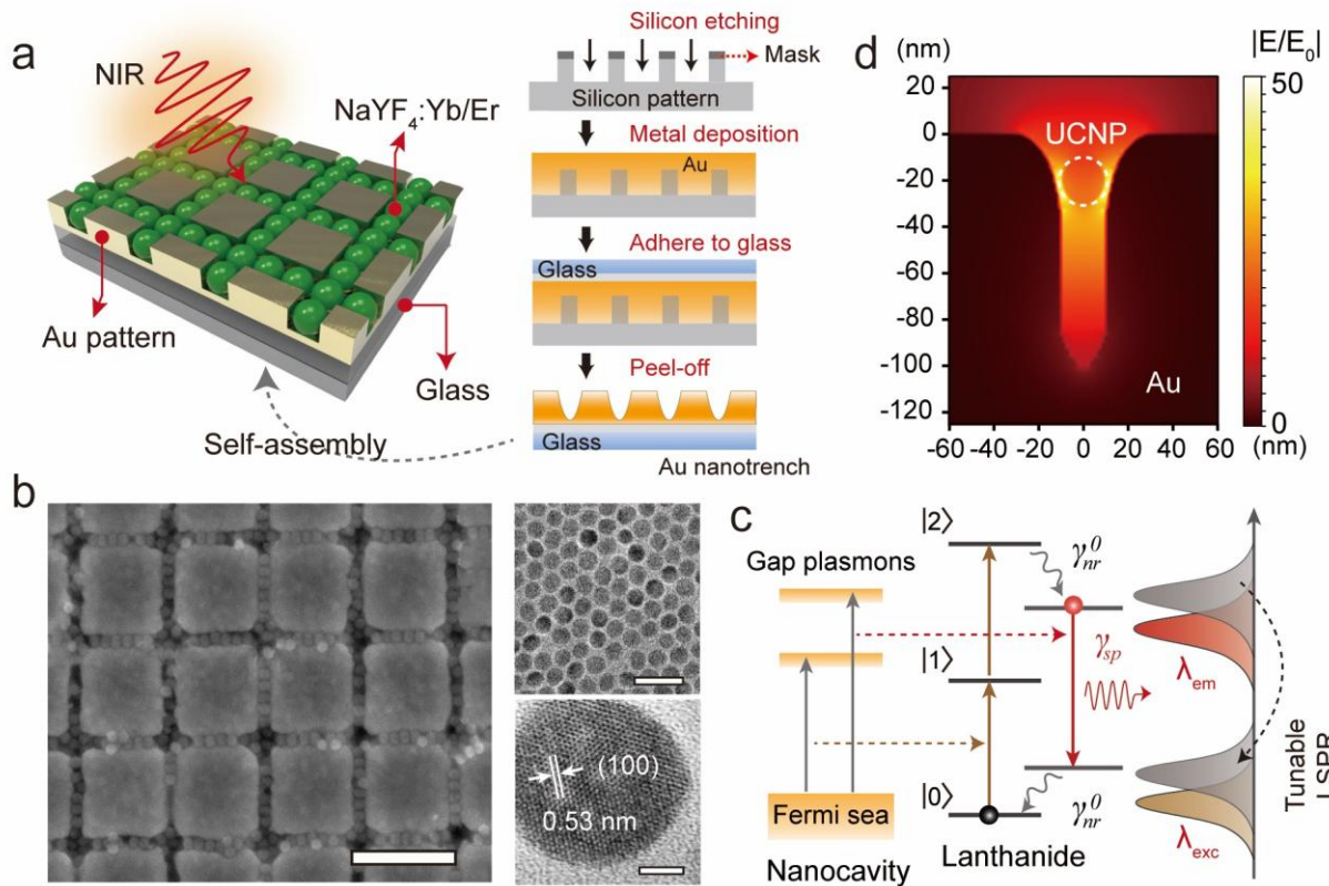
Figure 1. Upconversion emission enhancement through sub-wavelength confinement of optical fields. (a) Fabrication of gold nanotrenches (sub-20-nm gap) as plasmonic cavities for UCNPs. Briefly, hydrogen silsesquioxane resist was used to fabricate the mask for nanotrenches using electron beam lithography. The silicon substrate was then partially etched using inductively coupled plasma, followed by removing the resist through reactive ion etching. Next, a gold film with a thickness of 150-nm was deposited on the pre-patterned silicon substrate by e-beam evaporation. A glass slide adhered to the gold film using optical adhesive glue. After curing, the gold substrate comprising two-dimensional nanotrenches was peeled off. Lastly, UCNPs from the solution self-assembled into nanoscale gaps through capillary force. (b) Left panel: Scanning electron microscopy (SEM) image of UCNPs embedded in square arrays. Scale bar: 200 nm. Right panel: transmission electron microscopy (TEM) image of the as-synthesized \text{NaYF}_4:\text{Yb/Er} nanoparticles (scale bar: 50 nm) and high-resolution TEM image of a single nanoparticle (scale bar: 5
