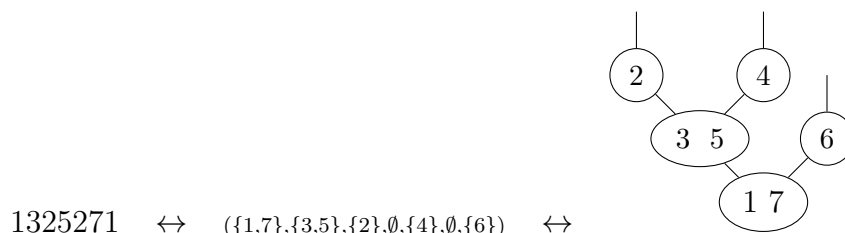
Figure 3: Bijection between parking functions, weak set compositions and parking trees.
