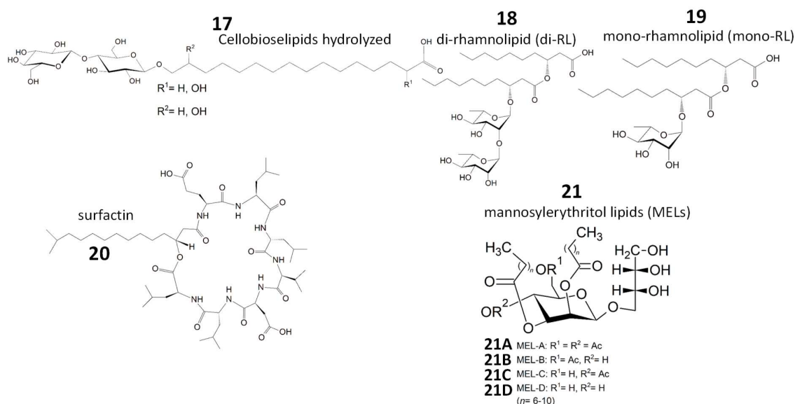
Figure 7 – Chemical structure of the main biosurfactant molecules presented in this review
