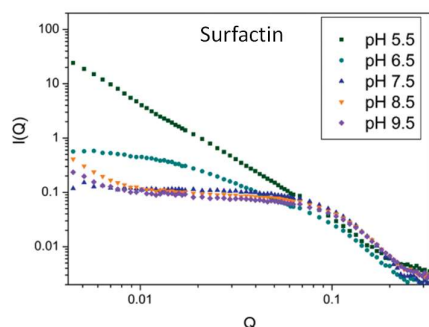
Figure 10 – pH-dependent SANS profiles recorded for surfactin (2 mM). Reprinted with permission from 212 . Copyright (2011) American Chemical Society.
