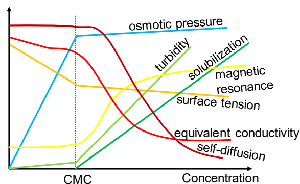
Figure 4 - Major properties employed in the study of critical micelle concentration. Image redrawn from B. Lindman and H. Wennerström, Topics in Current Chemistry, Vol. 87, Springer-Verlag, Berlin, 1980, p. 6.
