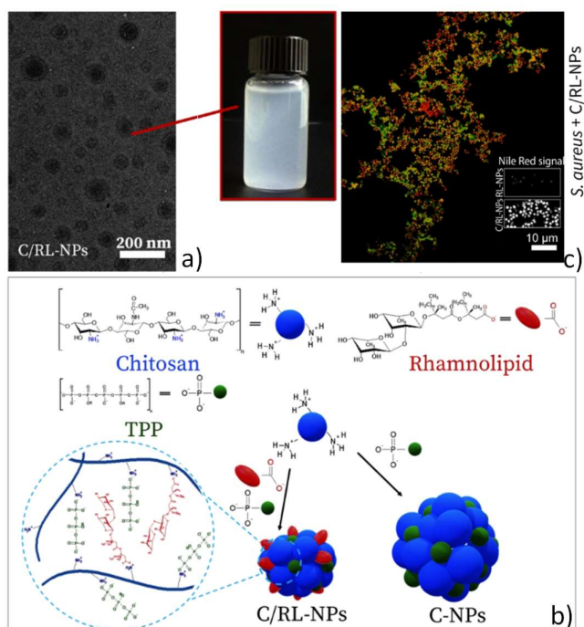
Figure 30 – a) Colloidally-stable chitosan-rhamnolipids ( 18 , 19 ) nanoparticles, b) their supposed structure and c) penetration into S. aureus (adapted with permission from 450 . Copyright 2020 American Chemical Society).
