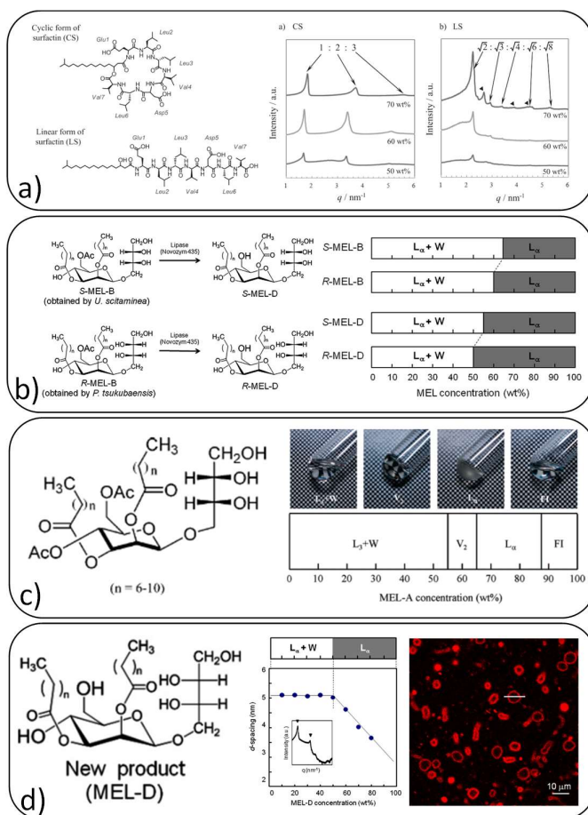
Figure 14 – Concentration-dependent phase diagrammes for a) surfactin (cyclic and linear) ( 20 ) (adapted from Ref. 282 , copyright Japan Oil Chemical Society), b) R- and S- MEL-B ( 21B ) and MEL-D ( 21D ) (reprinted from Ref. 225 with permission from Elsevier), c) MEL-A ( 21A ) (adapted with permission from Ref. 223 , copyright (2007) American Chemical Society), and d) MEL-D ( 21D ) (reprinted from Ref. 228 with permission from Elsevier). The L_{\alpha} +win b) and d) is associated to a MLV phase. Please refer to sections 2.3.3 and 2.3.4 for more explanation.
