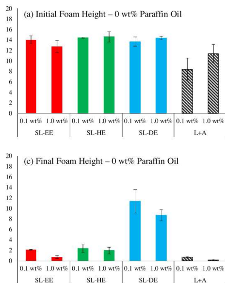
Figure 25 – Foaming properties of ester derivatives of ( 1 ) sophorolipids. SL-EE: ethyl ester SL, SL-HE: hexyl ester SL, SL-DE: decyl ester SL, L+A: 1:1 unmodified lactonic( 3 ):acidic( 1 ) SL mixture (Reprinted from 400 , Copyright (2016), with permission from Elsevier). The final foaming is measured after 60 min.
