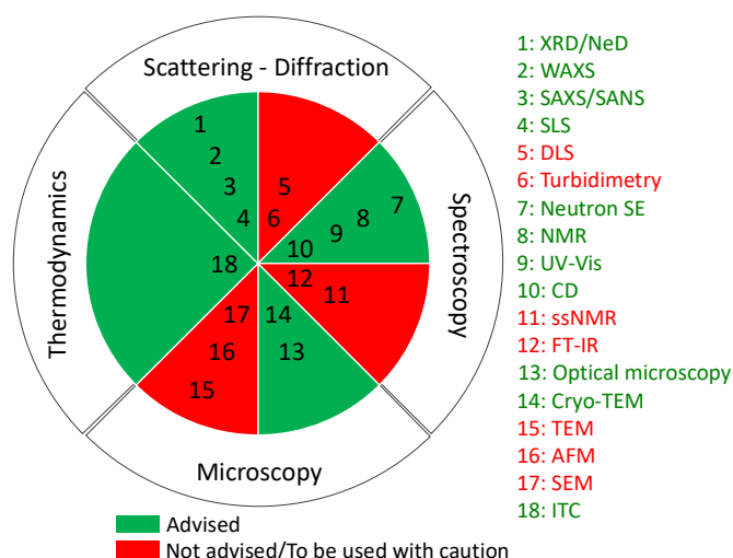
Figure 5 – List of the most common techniques, classified in four domains, employed in the study of amphiphile self-assembly in solution. Acronyms: SAXS (small-angle X-ray scattering), SANS (small-angle neutron scattering), SLS (static light scattering), Cryo-TEM (cryogenic transmission electron microscopy), TEM (transmission electron microscopy), SEM (scanning electron microscopy), AFM (atomic force microscopy), DLS (dynamic light scattering), XRD (X-ray diffraction), NeD (neutron diffraction), WAXS (wide-angle X-ray scattering), PL (polarized light microscopy), CD (circular dichroism), FT-IR (Fourier transform infrared spectroscopy), Neutron SE (neutron spin-echo), NMR (nuclear magnetic resonance), ITC (isothermal titration calorimetry), UV-Vis (ultra violet visible spectroscopy), ssNMR (solid state nuclear magnetic resonance)
