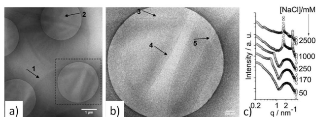
Figure 13 – a,b) Cryo-TEM of flat lamellar structures recorded for acidic glucolipid C18:0 (10) (0.5 wt%) at pH 7.8 and room temperature. Adapted with permission from 201 . Copyright (2016) American Chemical Society. c) NaCl-dependent evolution of the SAXS pattern recorded for a 5 wt% of the same compound (pH 7, RT). The high- q
