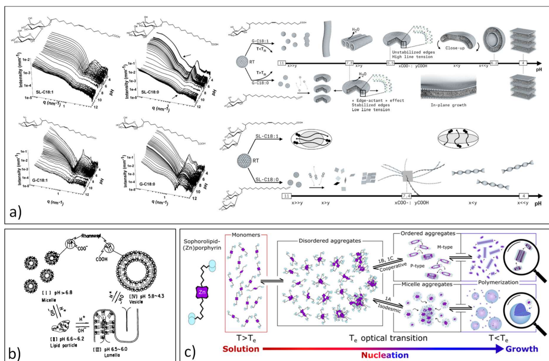
Figure 16 – pH-dependent phase transitions for a) nonacetylated acidic C18:1- cis ( 1 ), C18:0 sophoro ( 13 ) and glucolipids ( 10 ) 69 (adapted with permission from 69 . Copyright (2016) American Chemical Society) and b) rhamnolipids ( 18 , 19 ) (adapted with permission from 159 , copyright Japan Chemical Society). Temperature-dependent phase transition for porphyrin-derivative of sophorolipids ( 7 ). 209 (adapted with permission from 209 . Copyright (2019) American Chemical Society).
