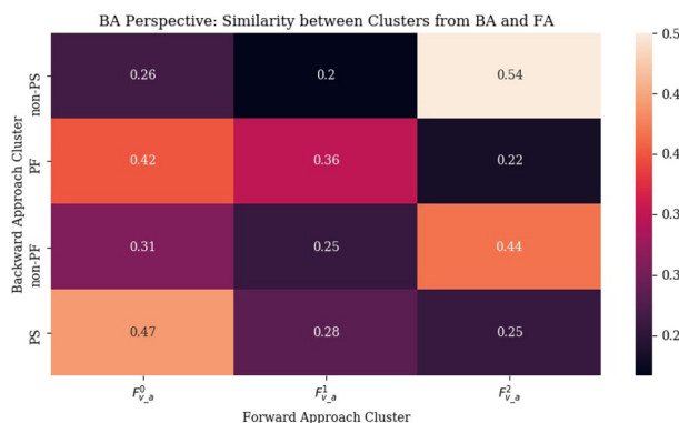
Fig. 15 Similarity Matrix between the clusters computed on the learning outcomes and performance metric (backward analysis - rows) and those computed on the video and audio features listed in the middle and bottom sections of Table 1 (forward analysis - columns)
