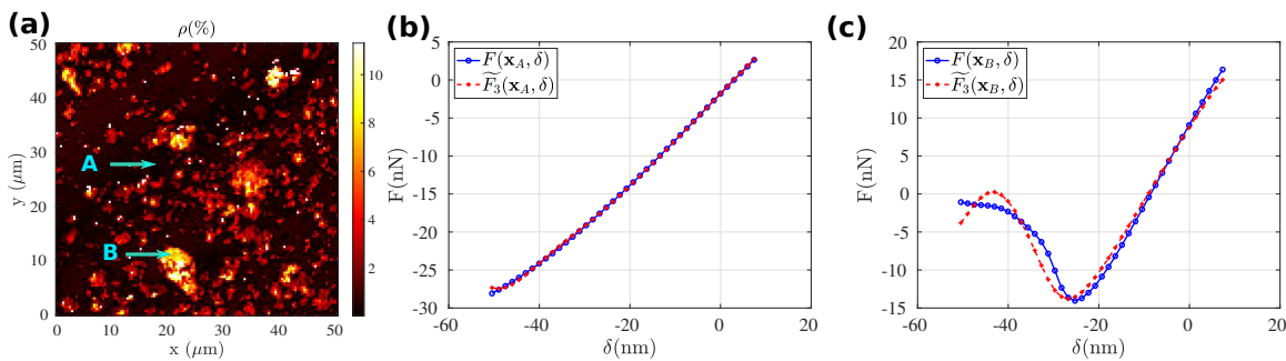
Figure 5: Uncertainty(residual) of reconstruction using the first three POD modes: (a) The residual map ; (b) Comparison between the initial force-indentation curve (plotted in dot blue) and reconstructed curve (plotted in red) at point A ( \rho(\mathbf{x}_A) \simeq 1\% ); (c) Comparison between the initial force-indentation curve (plotted in dot blue) and reconstructed curve (plotted in red) at point B ( \rho(\mathbf{x}_B) \simeq 10\% )
