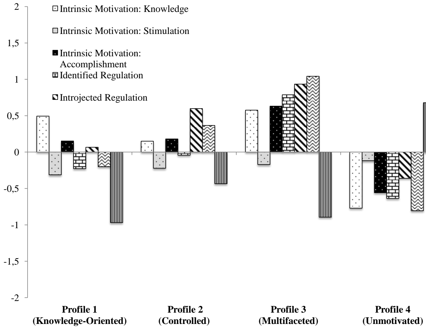
Figure 1. Final Latent Profile Solution.
