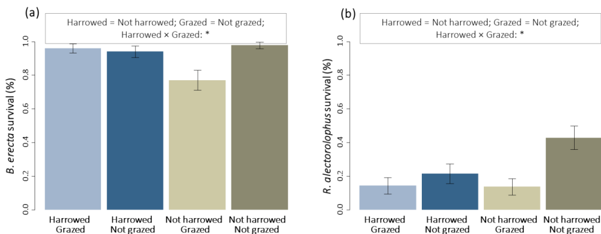
14 Fig. 4. Final seedling survival of (a) Bromopsis erecta and (b) Rhinanthus alectorolophus . The 15 direction of main effects is indicated using "<" ( P < 0.05 ) and "=" (not significantly different). 16 Significant grazing-by-soil preparation interactions are presented using "*" ( P < 0.05 ).
