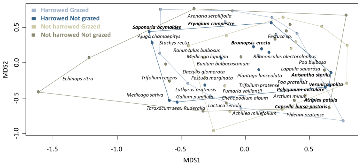
9 10 Fig. 3. Plant species composition in the four restoration treatments using NMDS. Polygons 11 indicate the position of the outmost plots in each treatment (NMDS stress: 0.190).
