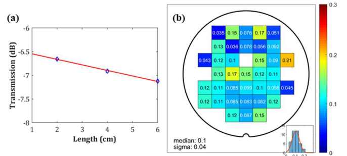
Fig. 4: C-band propagation loss measurement. (a) Maximum transmission of spiraled rib waveguides as a function of their length (blue diamond) and linear fit giving the propagation loss of the smoothed rib waveguide (red line). (b) Wafer scale mapping of smoothed rib waveguide propagation losses at 1550 nm (in dB/cm).
