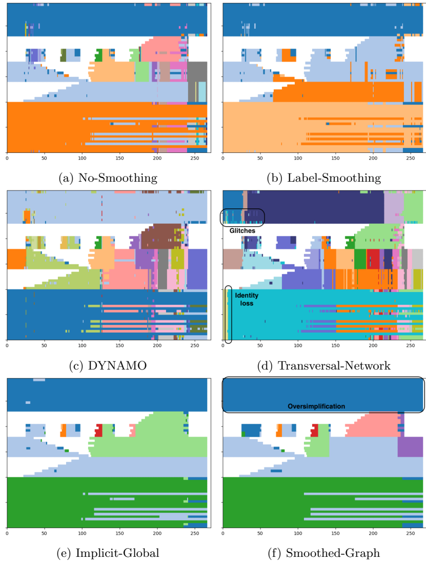
Figure 6: Comparison of partitions obtained using all methods on the ad-hoc scenario, blurred variant. We annotated examples of typical smoothing problems: Glitches, Identity loss and Oversimplification
