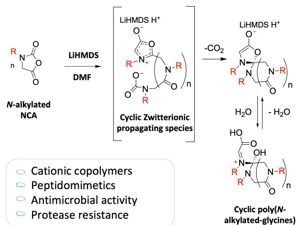
Scheme 1. LiHMDS-mediated REP of NNCA: cyclic and bioactive species are produced in a controlled fashion.
