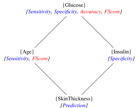
Fig. 4: The interpretation of the 4 important features in the Pima Indians Diabetes dataset. For the sake of legibility, only the most specific terms describing the sets of features are depicted. Terms are written in blue if they are related to prediction and in red if they are related to discrimination.
