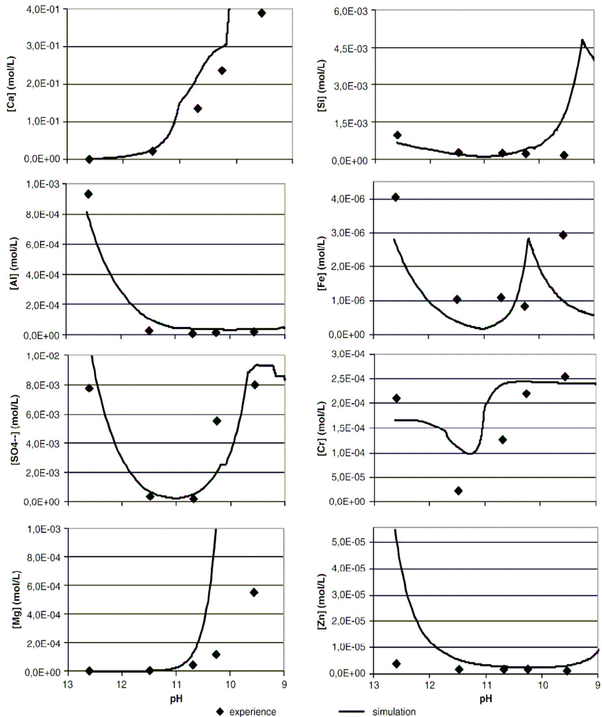
Figure 5. Experimental and simulated leaching curves of OPC-PFA-S.
