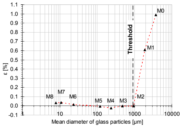
Figure 1. Influence of glass particle size on expansion
