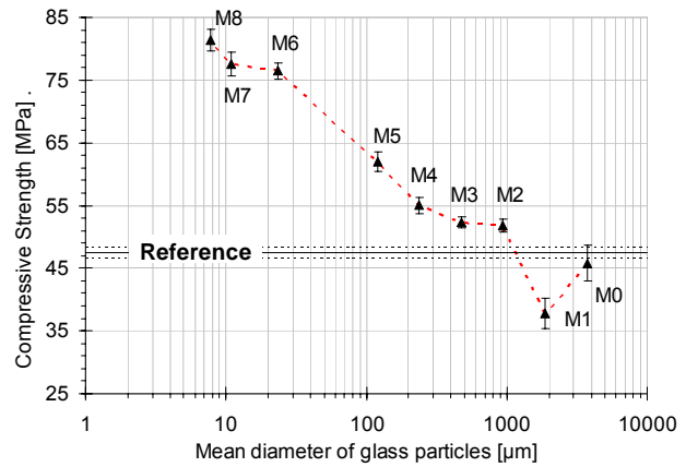
Figure 2. Influence of glass particle size on compressive strength development
