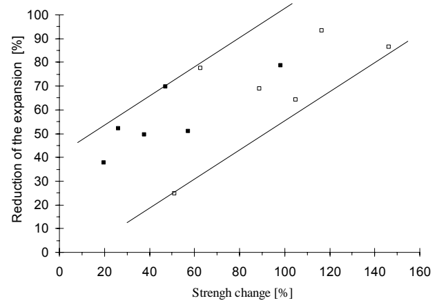
Figure 5. Reduction of expansions with increased compressive strength of mortars containing fine particles of glass
