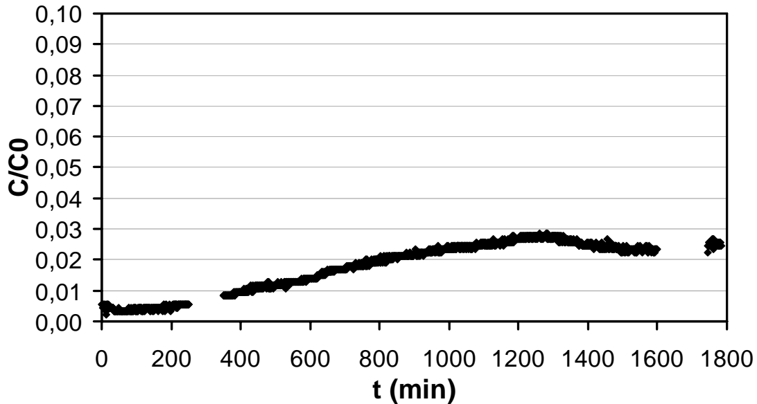
Figure 3. H 2 S adsorption breakthrough curve on MSWI-BA-A material containing 18%wt moisture and packed in fixed bed
