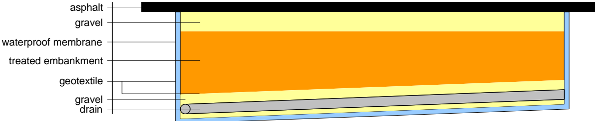
Figure 5 – Profile of road structure for the test of lime-based binder used in treated embankment.
