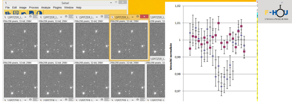
FIG. 2. Modeling activities on the detection of an exoplanet. The real problem is provided by a series of image of the same field taken at regular time interval ( left ). The model used is that of a star and an exoplanet orbiting around it. The mathematical prediction of the model is a graph showing the evolution with time of the luminosity of different stars in the field ( right ).
