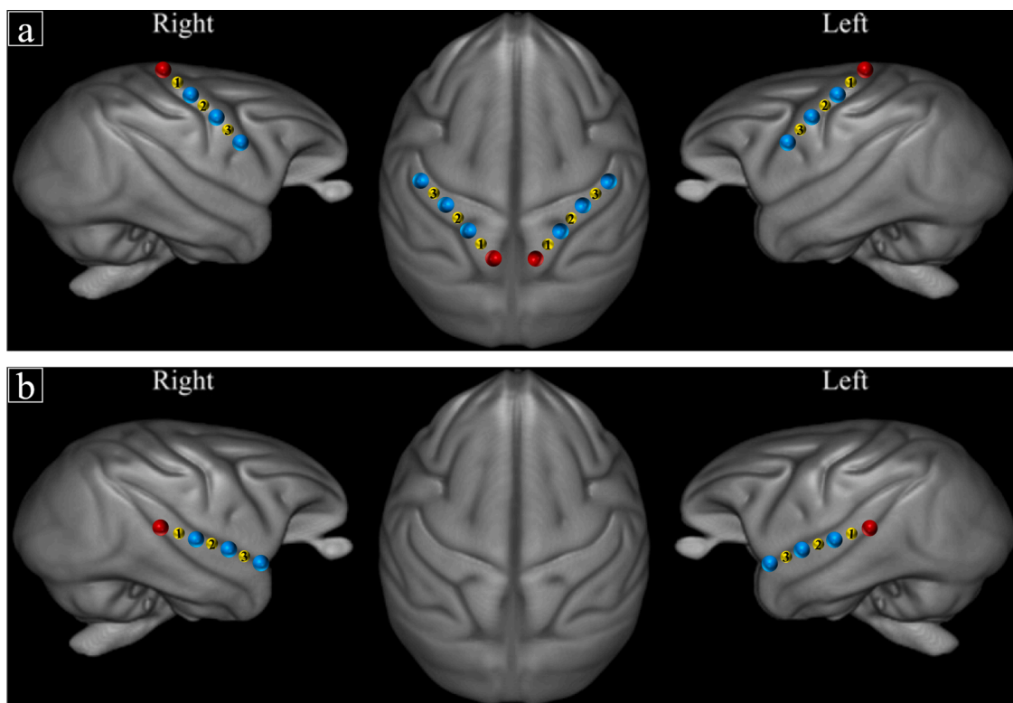
Fig. 1. Schematic representation of fNIRS channel locations on ROIs according to T1 MRI template from 89 baboons [60] for (a) the sensorimotor and (b) the auditory stimulations. Red and blue dots indicate the positions of the receivers and transmitters respectively. Yellow dots indicate channel numbers.
