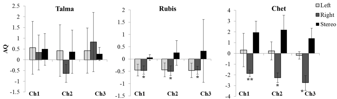
Fig. 3. Normalized averaged AQ (and corresponding SE) above the temporal cortex following auditory stimulations in three adult female baboons (see Fig. 1 for localization of the channels). All AQs were normalized using the scale function of R studio (R studio (2015) Inc., Boston, MA, url: http://www.rstudio.com/ ). In an absolute perspective, positive values correspond to right hemisphere activation. In a relative perspective, more positive values correspond to more rightward differences in activation. \mu \neq 0 at p < 0.05^* and p < 0.01^{**} .
