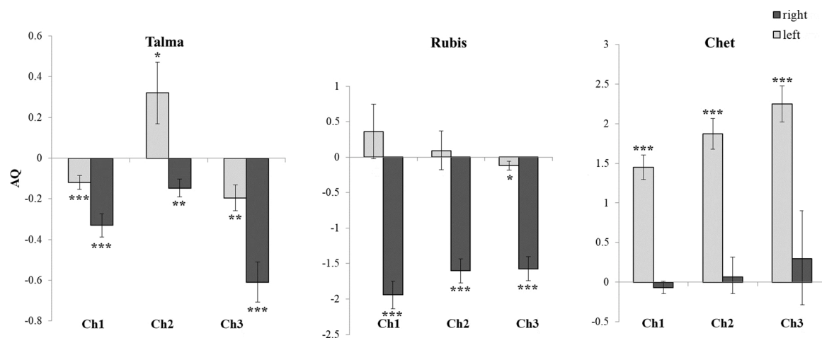
Fig. 2. Normalized averaged AQ (and corresponding SE) in the motor cortex following sensorimotor stimulations in the three adult female baboons (see Fig. 1 for localization of the channels). All AQs were normalized using the scale function of R studio (R studio (2015) Inc., Boston, MA, url: http://www.rstudio.com/ ). In an absolute perspective, positive values correspond to right hemisphere activation. In a relative perspective, more positive values correspond to more rightward differences in activation. \mu \neq 0 at p < 0.05^* , p < 0.01^{**} and p < 0.001^{***} .
