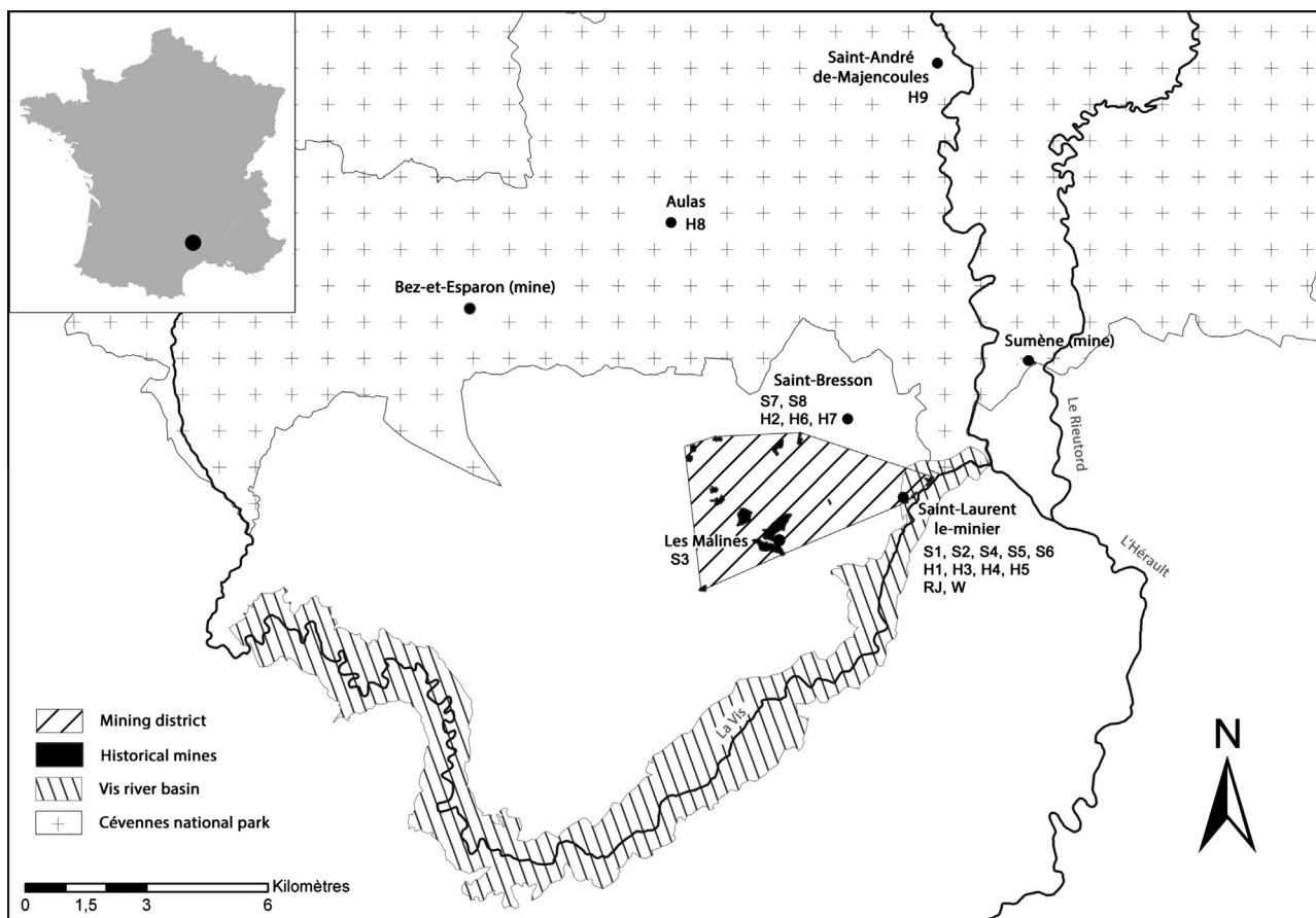
Fig. 1. Location of historical mines and sampling sites (sample names in accord with Table 2 and 3).
