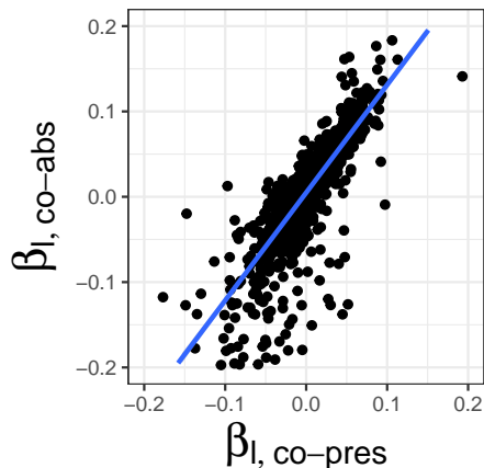
Figure S.23: Results of ELGRIN on the European tetrapods case study. The parameters \beta_{l,co-pres} and \beta_{l,co-abs} were highly correlated.
