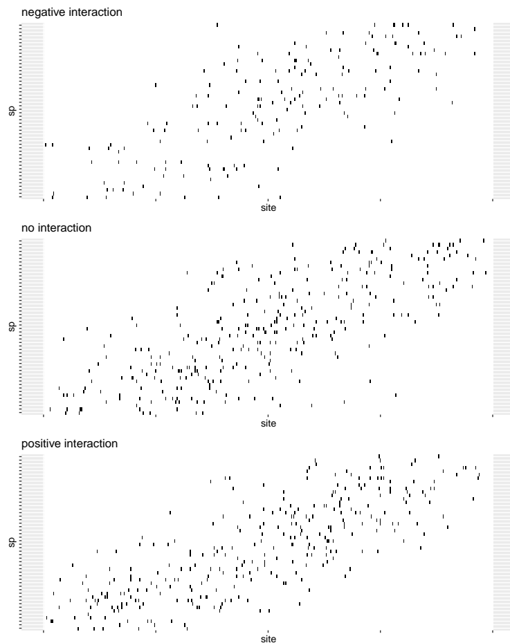
Figure S.19: Presence-absence of species ( y -axis) along the environmental gradient ( x -axis) for the Lotka-Volterra simulations with intraspecific interactions larger than interspecific ones, across the three interaction scenarios.
