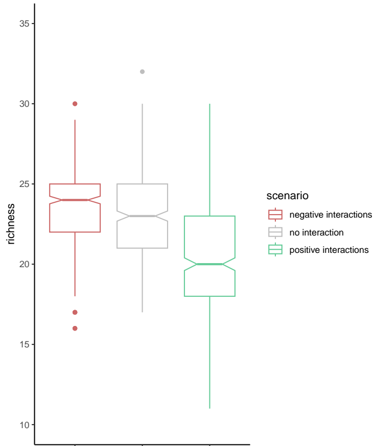
Figure S.17: Distribution of species richness (observed number of present species) for the Virtual-Com simulation under the three interaction scenarios.
